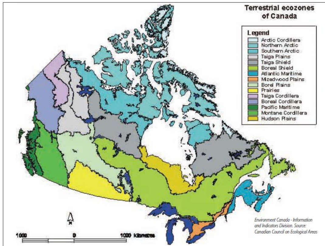
Figure A1. The Terrestrial Ecozones of Canada (Environment Canada, 1996; Kull et al. , 2006).
